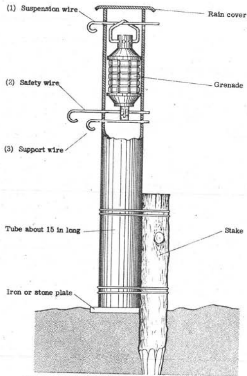
Figure 118. Tube-type booby trap.
