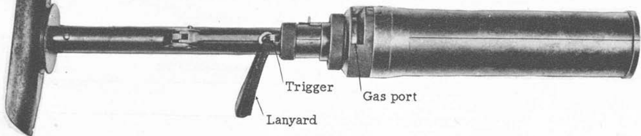
Figure 51. Model 10 (1921) 50-mm grenade discharger.
