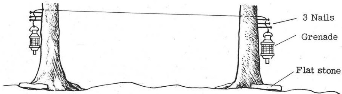
Figure 120. Use of grenades in booby trap, with string stretched between trees.
