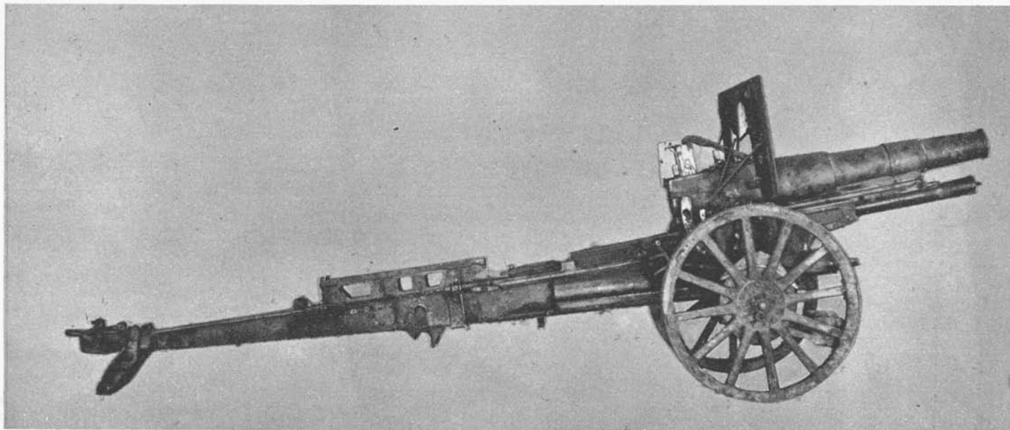
Figure 85. Model 4 (1915) 150-mm howitzer.
