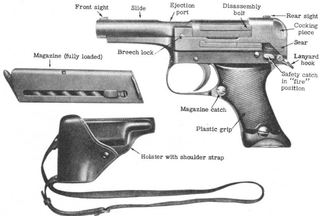
Figure 35. Model 94 (1934) 8-mm pistol, magazine and holster.
