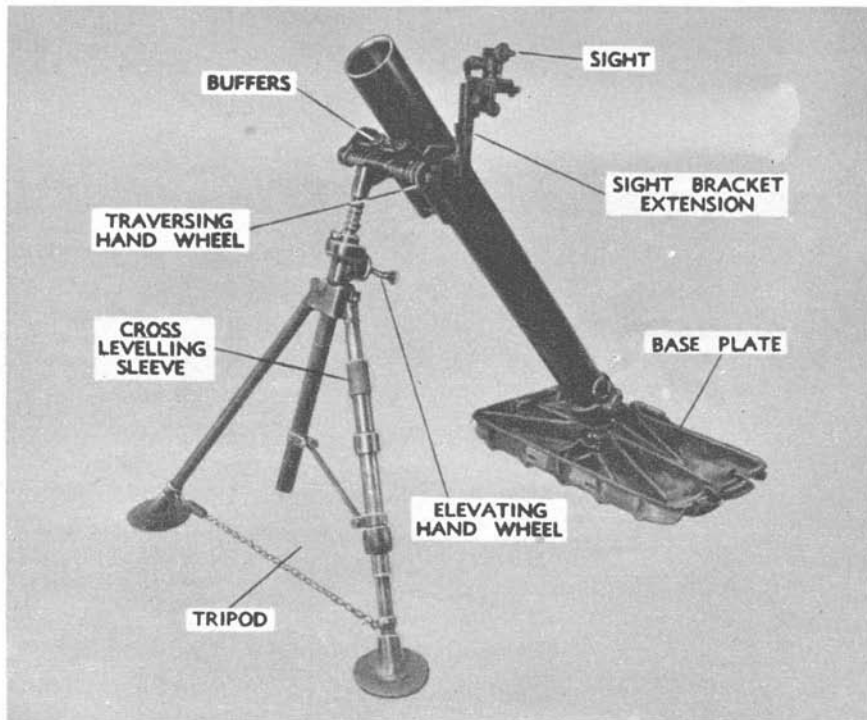
Figure 67. Model 97 (1937) 90-mm mortar.
