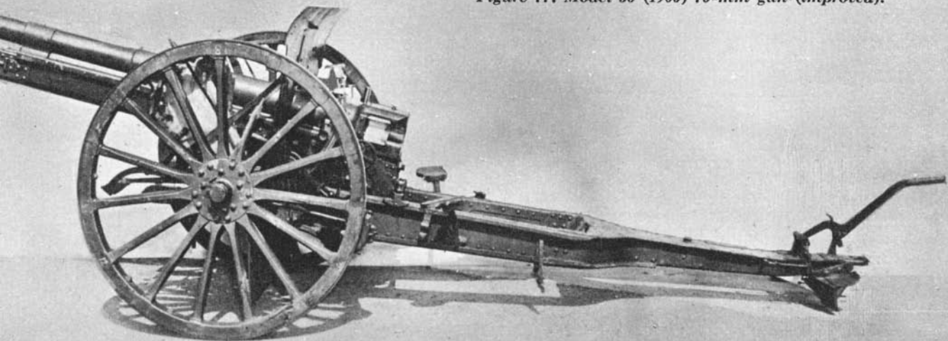
Figure 77. Model 38 (1905) 75-mm gun (improved).
