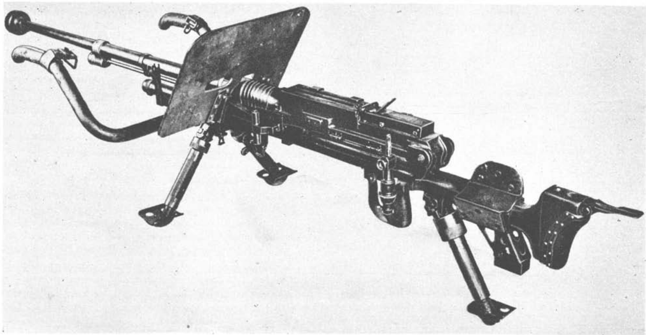
Figure 69. Model 97 (1937) 20-mm antitank rifle with shield and front carrying handles.
