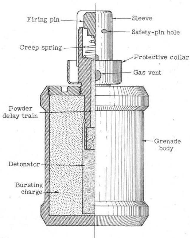
Figure 45. Model 99 (1939) "Kiska" hand grenade.
