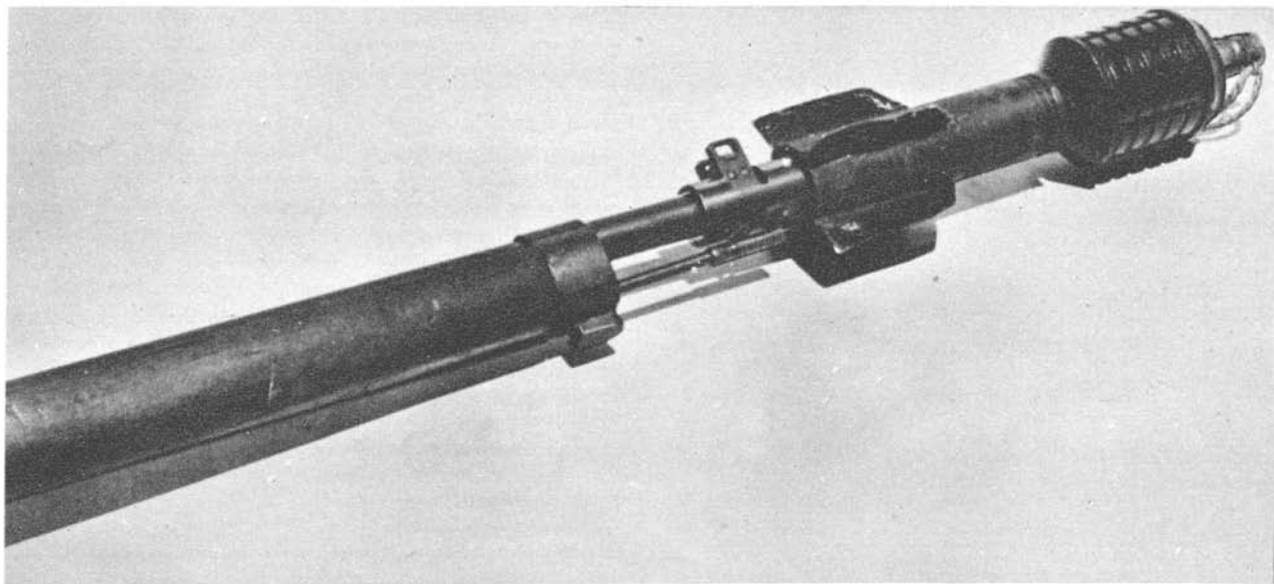
Figure 40. Spigot-type grenade launcher.
