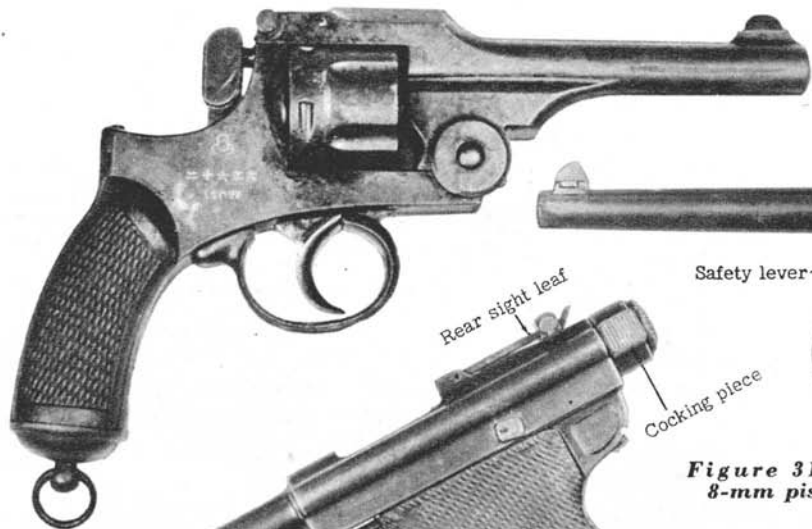
Figure 30. Model 26 (1893) 9-mm revolver (left).
