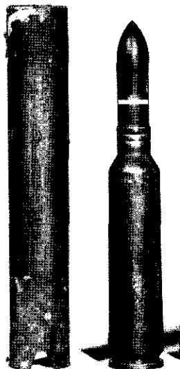
Figure 116.—20-mm armor-piercing round with cardboard container.
