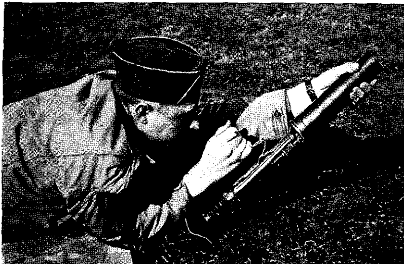
Figure 47.—Firing Model 89 (1929) 50-mm grenade discharger from prone position.
